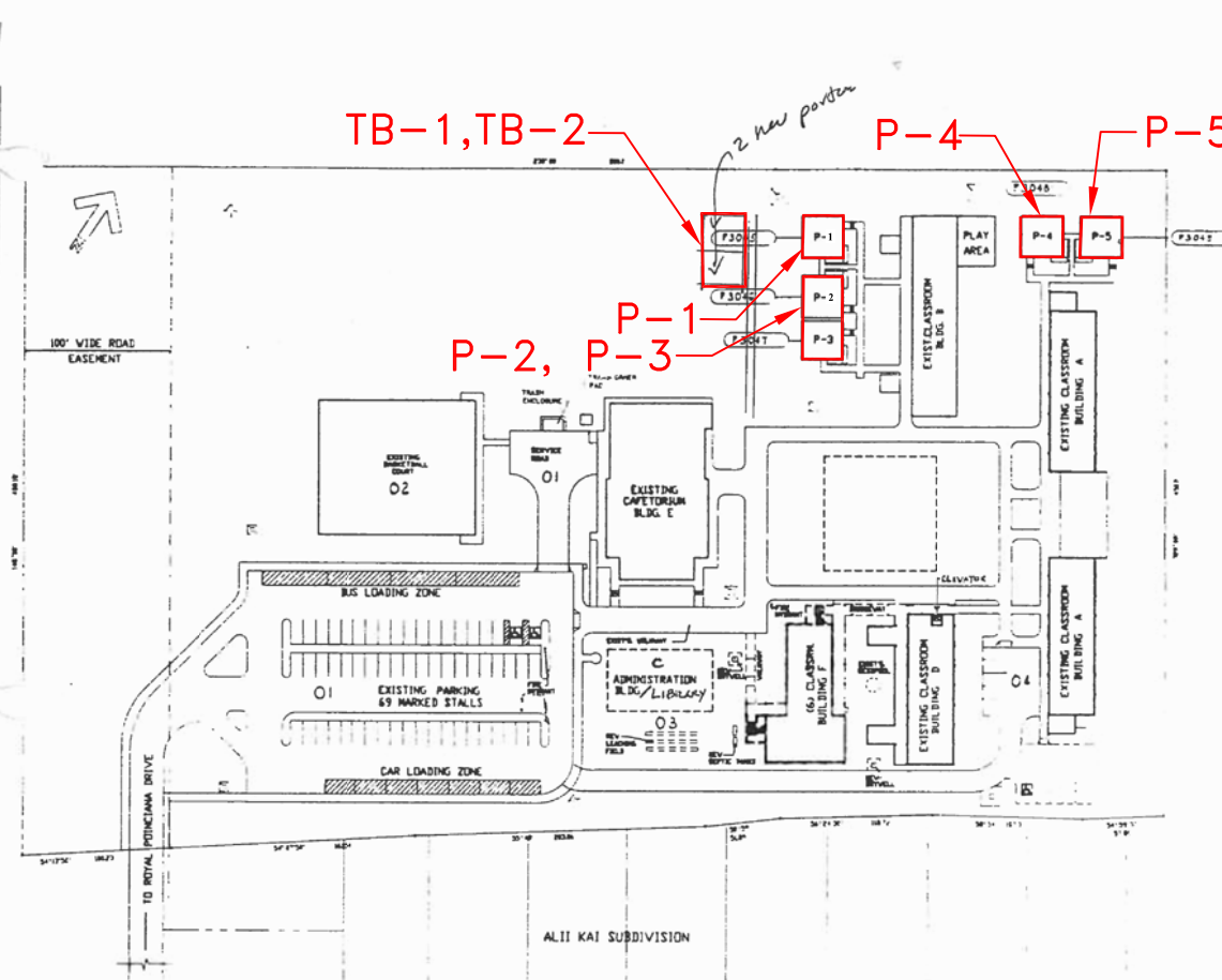
PROJECT PLOT PLAN SCALE: 1" = 40'-0"
